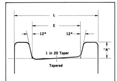
Standard Double Flanged Crane Wheels for Rail Lighter than the Three Special Crane Rail Sizes
